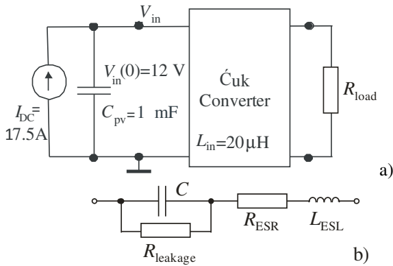
Figure 6. a) Simplified model of the PV system used to excite the Ćuk converter with large capacitance in between. b) Model of the electrolytic capacitor ( C_{pv} ): C=1mF , R_{leakage}=1 M\Omega , R_{ESR}=0.5 \Omega , and L_{ESL}=3 nH .
