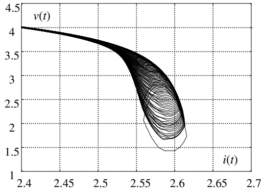
Figure 9. Chaotic diagram representing the current voltage relationship at the PV panel - converter interface for I_p=1.3 A
