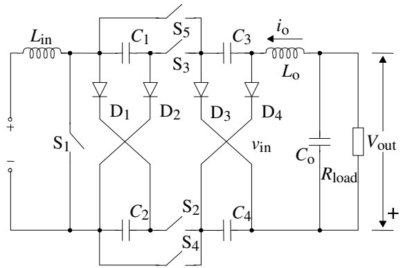
Figure 4. The Ćuk converter
