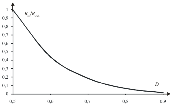
Figure 5. Normalized input resistance of the converter as a function of the duty cycle
